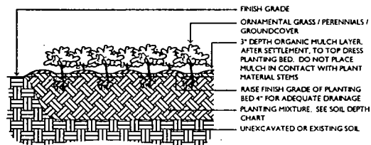
3 GROUND COVER/PERENNIAL INSTALLATION DETAIL 3/4" = 1'-0"
