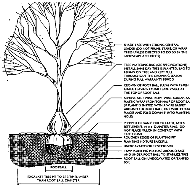
2 TREE INSTALLATION DETAIL 3/4" = 1'-0"
