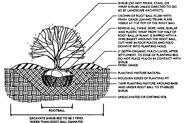
4 SHRUB INSTALLATION DETAIL 3/4" = 1'-0"
