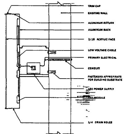
Standard Face Lit LED Illuminated w/ Raceway
