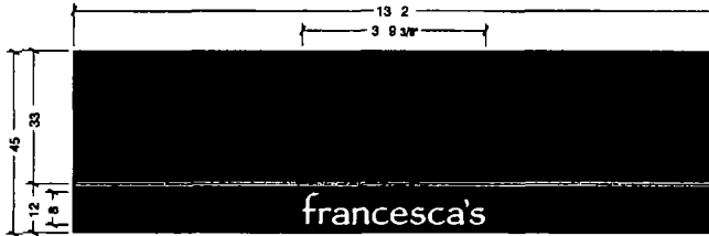
A AWNING DETAIL 2 SCALE 1/2" = 1' 0" QTY 1
