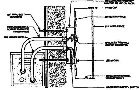
Typical U.L. Channel Letter Set Mounted on Wireway
