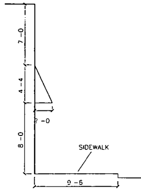
○ 4617 N KEDZIE — SECTION VIEW SCALE 1/8" = 1'-0"
