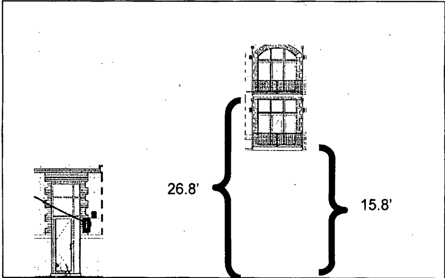
W. Hubbard St. Elevation (South Elevation) – 2 balconies
