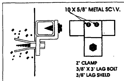
FRAME TO WALL ANCHOR DETAIL
