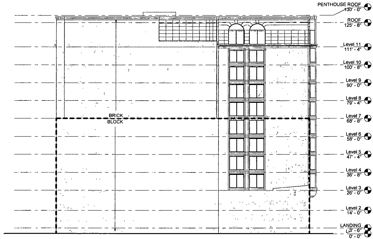
① SOUTH ELEVATION - SUB AREA "A" 1/16" = 1'-0"
