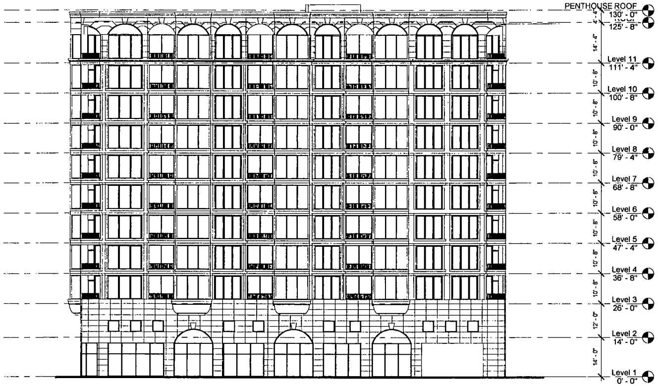
① NORTH ELEVATION - SUB AREA "A" 1/16" = 1'-0"
