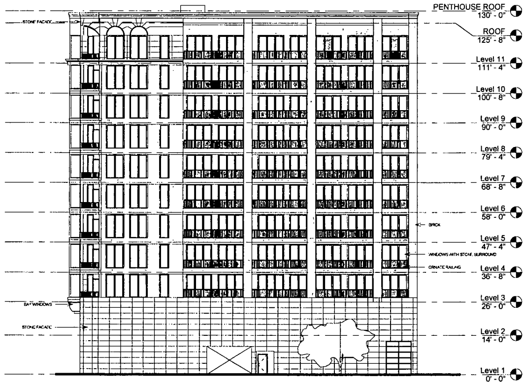
① WEST ELEVATION - SUB AREA "A" 1/16" = 1'-0"
