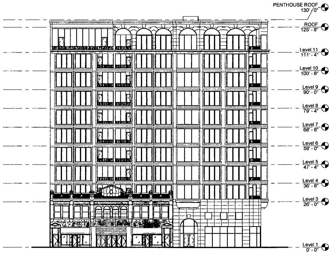
① EAST ELEVATION - SUB AREA "A" 1/16" = 1'-0"
