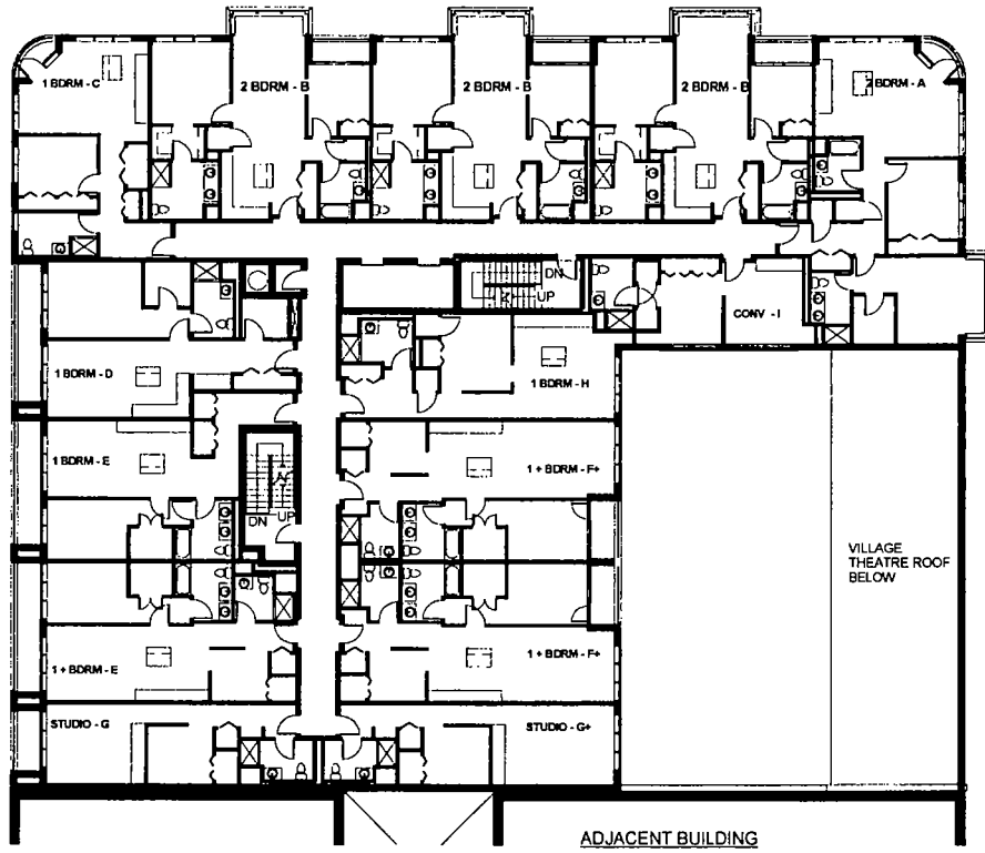
① 3RD - 10TH FLOOR PLAN 1/16" = 1'-0"
