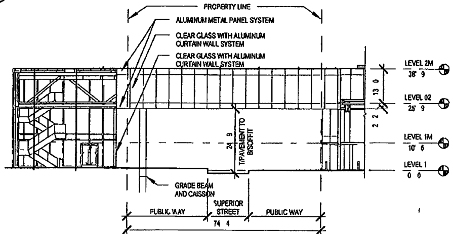
3 WEST ELEVATION
