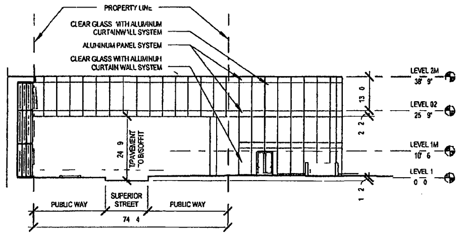
1 EAST ELEVATION
