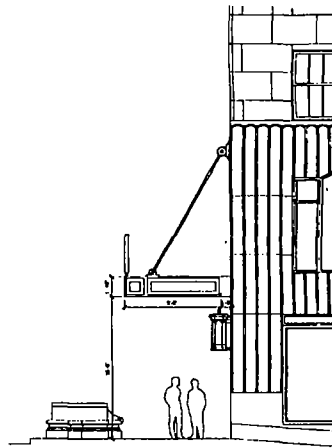
2 EAST ELEVATION SCALE 1/4"=1'-0"
