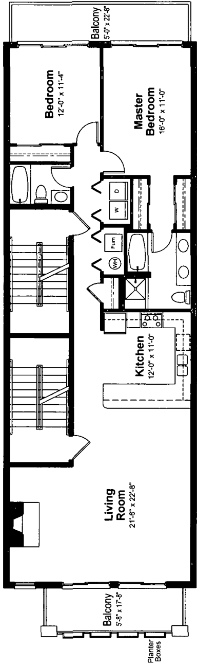
2nd, 3rd, and 4th Floor Plan
