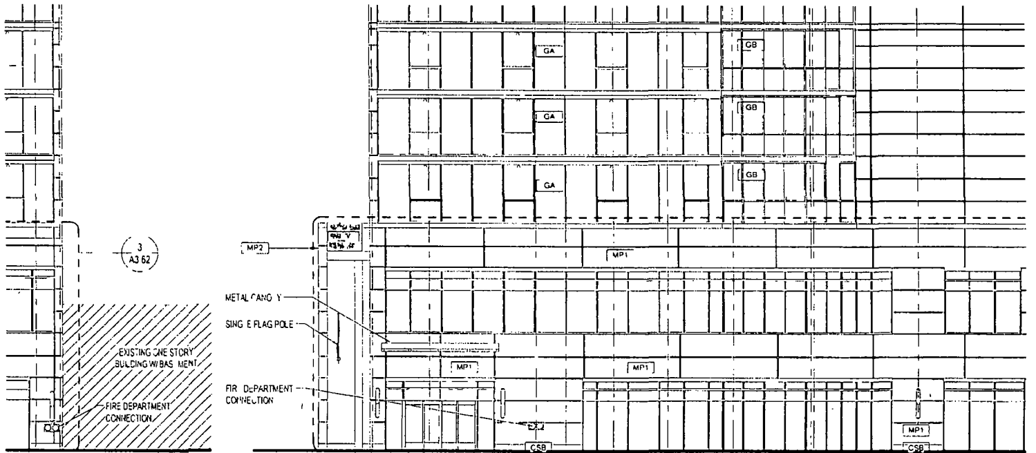
1 SOUTH ELEVATION (HL) 16 1-4
