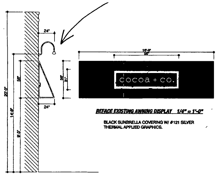
SIDE VIEW 1/4" = 1'-0"
