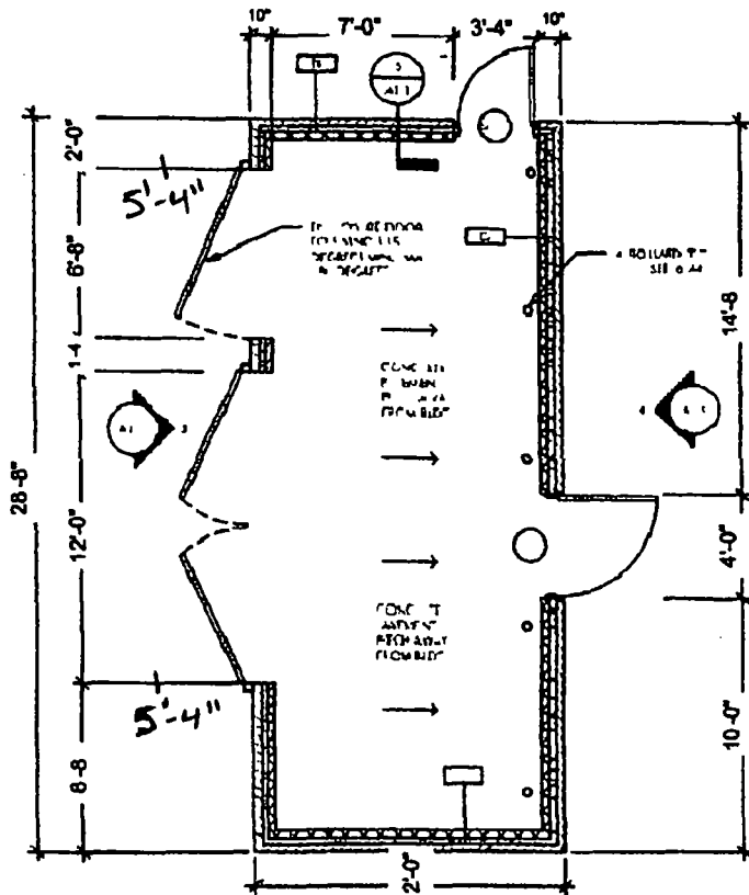
2 TRASH ENCLOSURE PLAN
