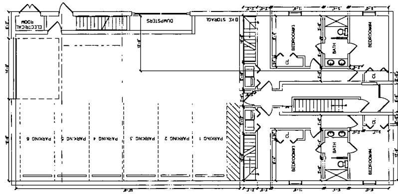
① 1ST FLOOR LEVEL-PROPOSED 3/32" = 1'-0"
