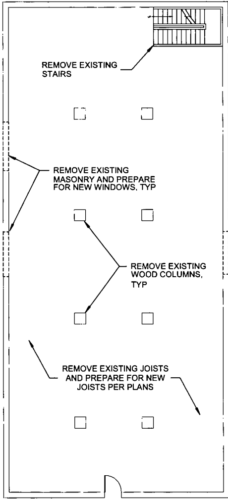
① 1ST FLOOR LEVEL- EXISTING 3/32" = 1'-0"
