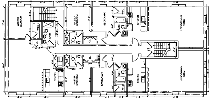
③ 3RD FLOOR LEVEL-PROPOSED 3/32" = 1'-0"
