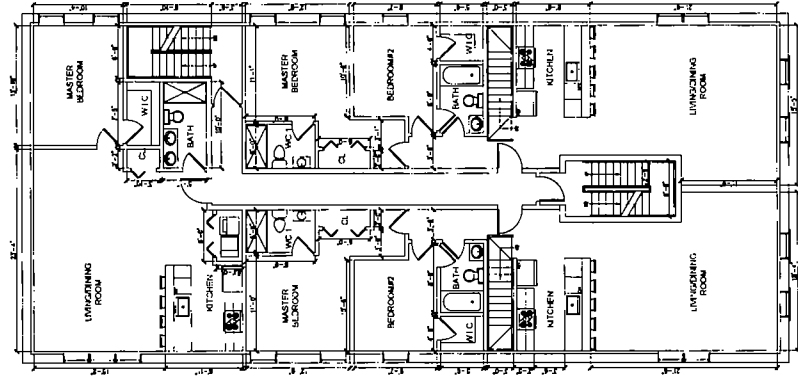
② 2ND FLOOR LEVEL-PROPOSED 3/32" = 1'-0"
