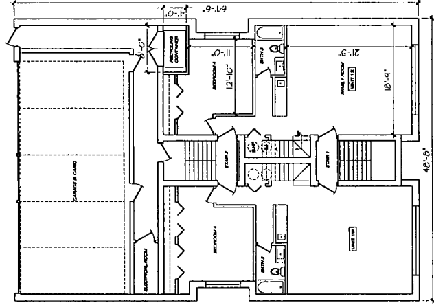
BASEMENT/GARAGE FLOOR PLAN
