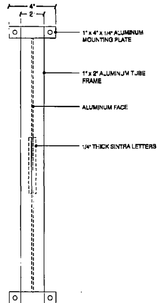
CROSS SECTION NTS
