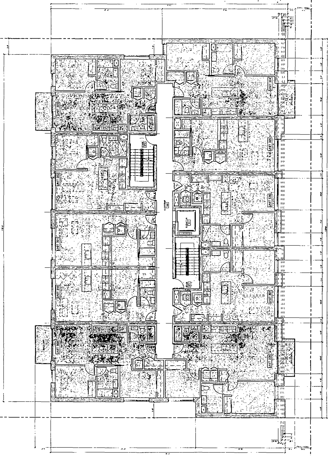
3/16" = 1'-0" N LEVEL 3 FLOOR PLAN 3431 N. ASHLAND
