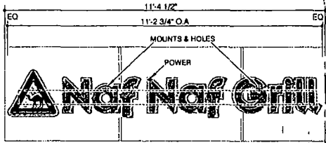
INDIVIDUAL INT. LED ILLUMINATED LETTER DISPLAY 3/8" = 1'-0"
