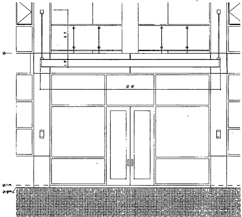
ENTRANCE CANOPY ELEVATION DETAIL
