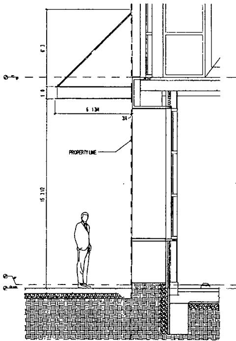
ENTRANCE CANOPY SECTION DETAIL
