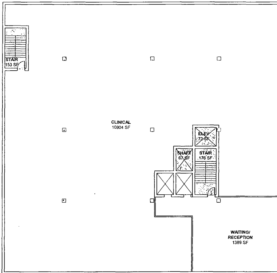
FLOORS 4-7
