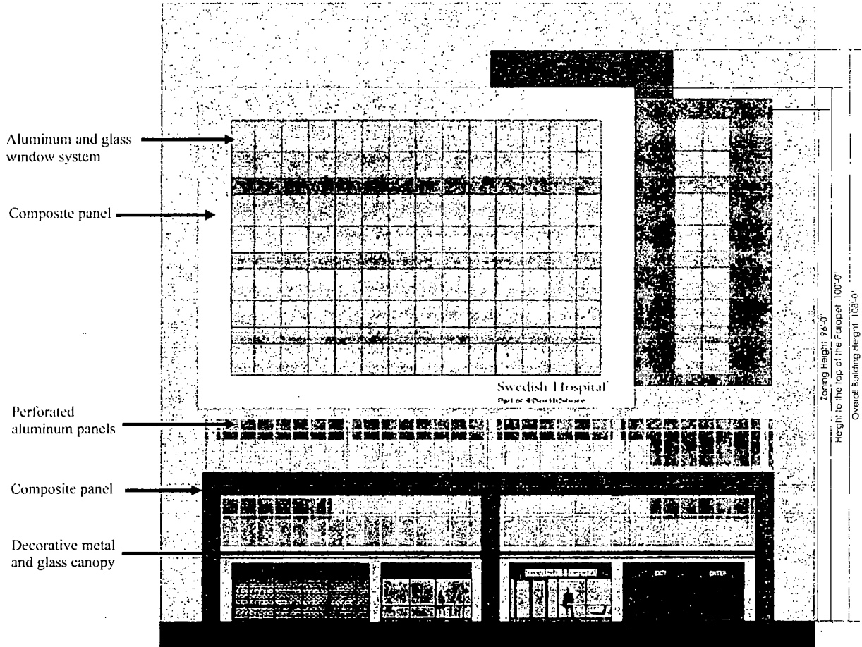
SOUTH ELEVATION
