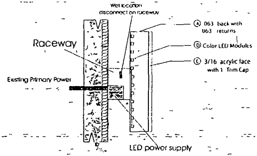
Typical Raceway Mount channel Letters with LED s
