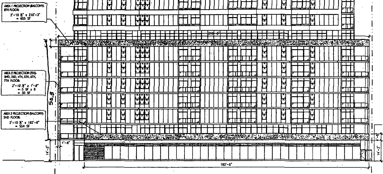
EAST ELEVATION - 1/16" = 1'-0"
