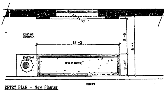
ENTRY PLAN - New Planter
