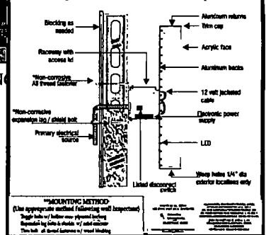
LED CHANNEL - RACEWAY MOUNT
