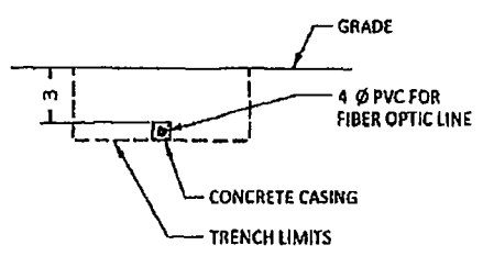
FIBER OPTIC LINE - TYPICAL SECTION
