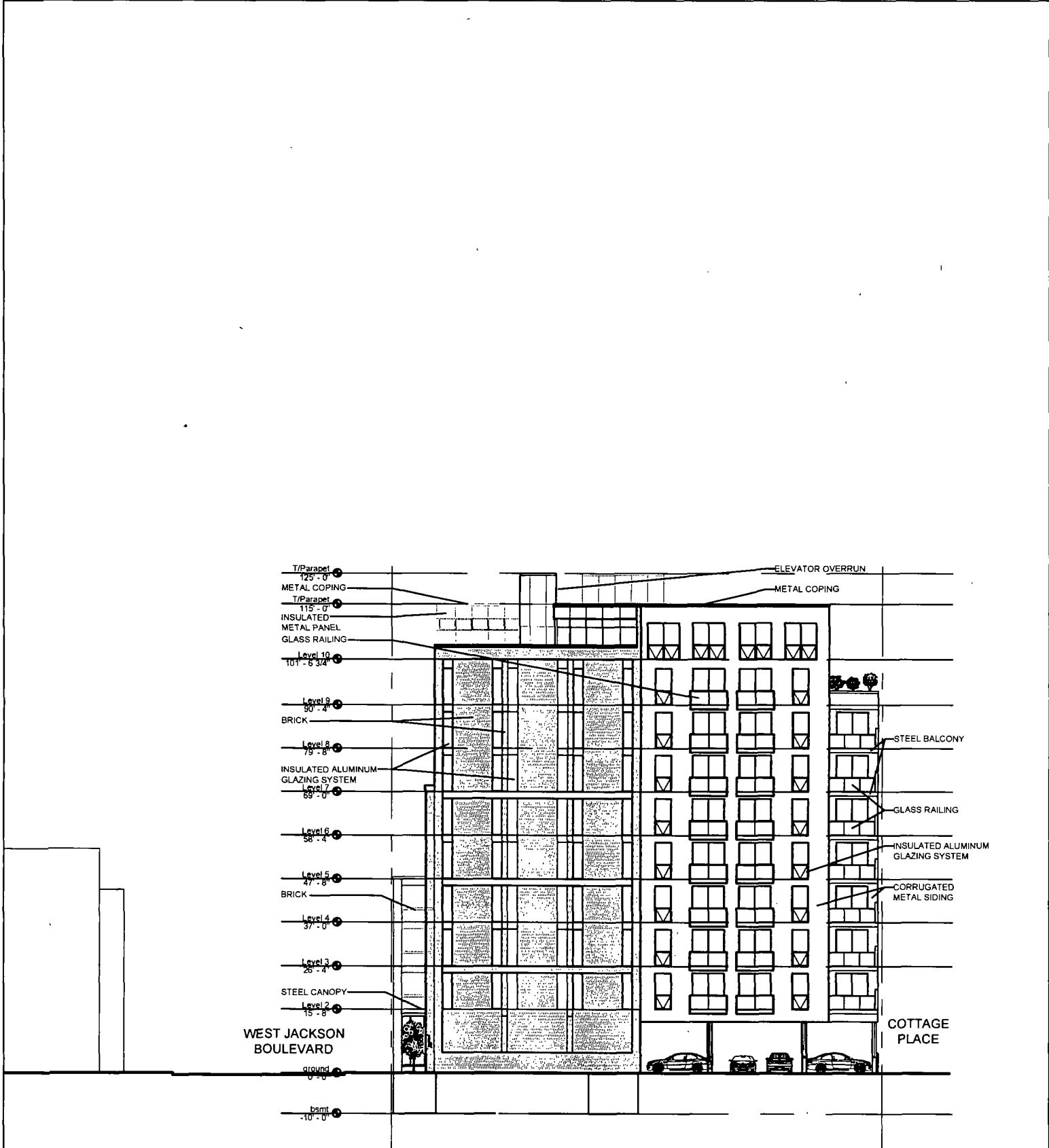
EAST ELEVATION SCALE: 1/32" = 1'-0"
