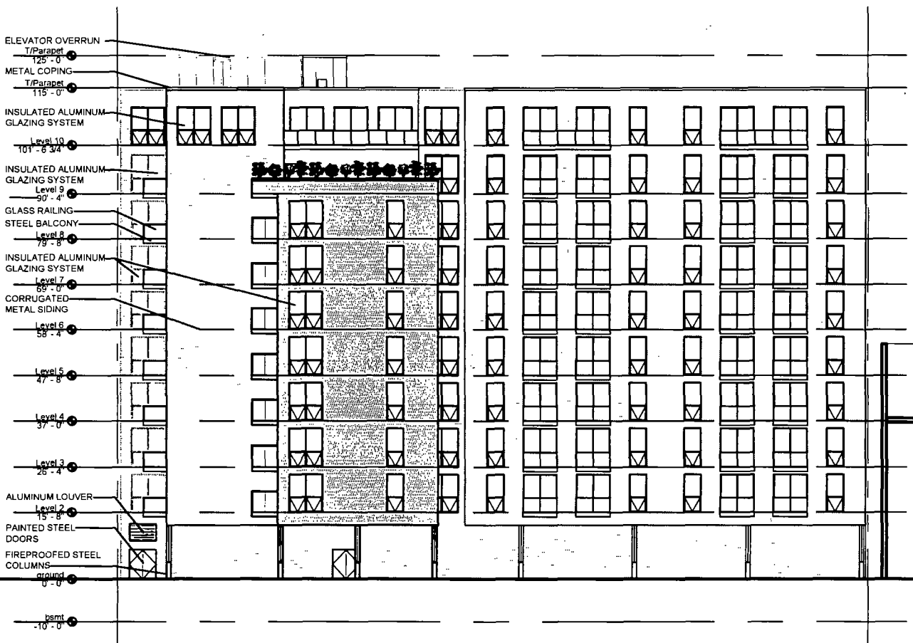
NORTH ELEVATION (ALLEY) SCALE: 1/32" = 1'-0"
