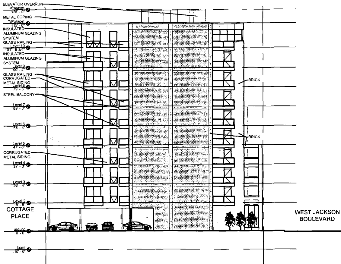
WEST ELEVATION SCALE: 1/32" = 1'-0"
