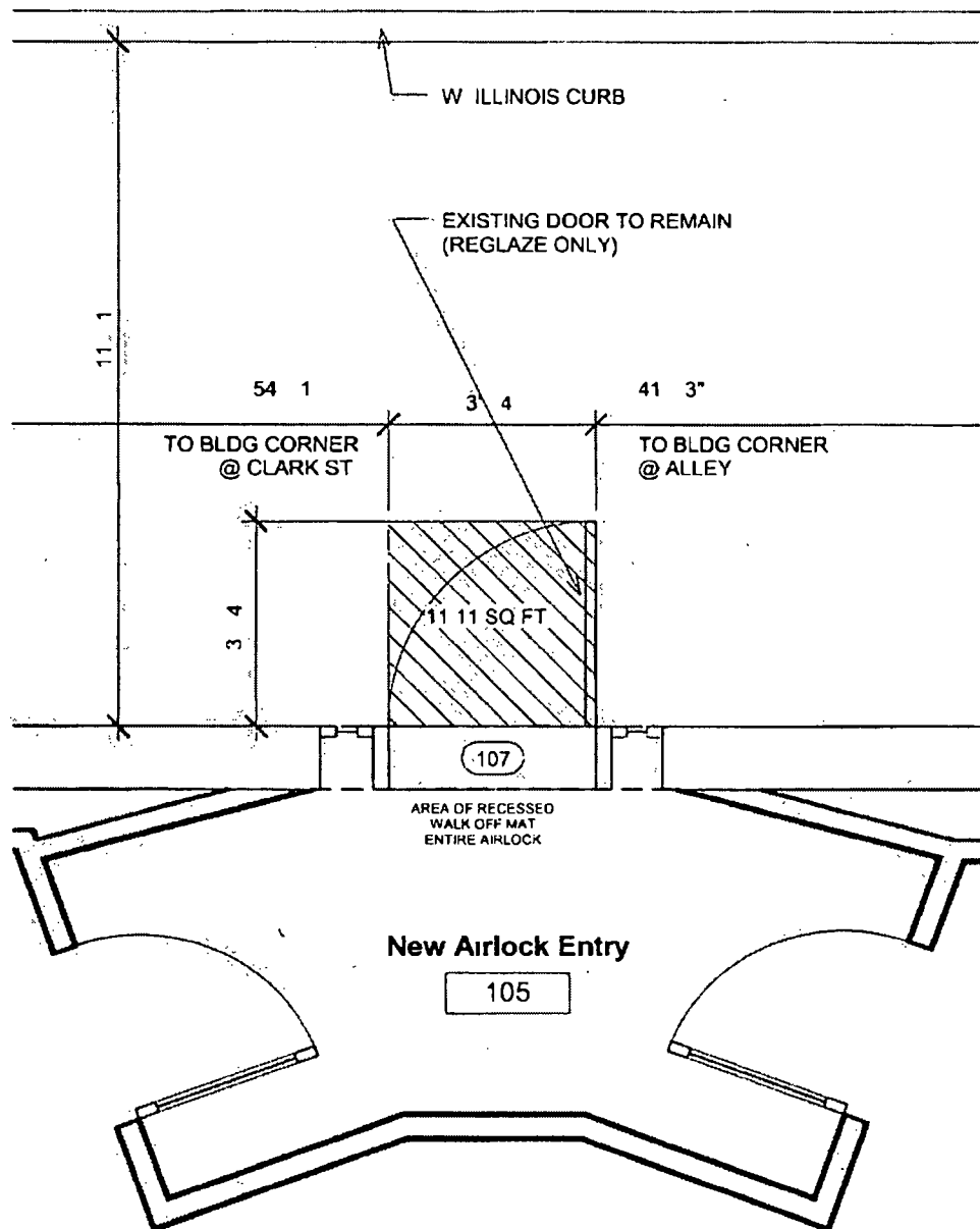
① 1st Floor, Door 107 Diagram 3/8" = 1'-0"
