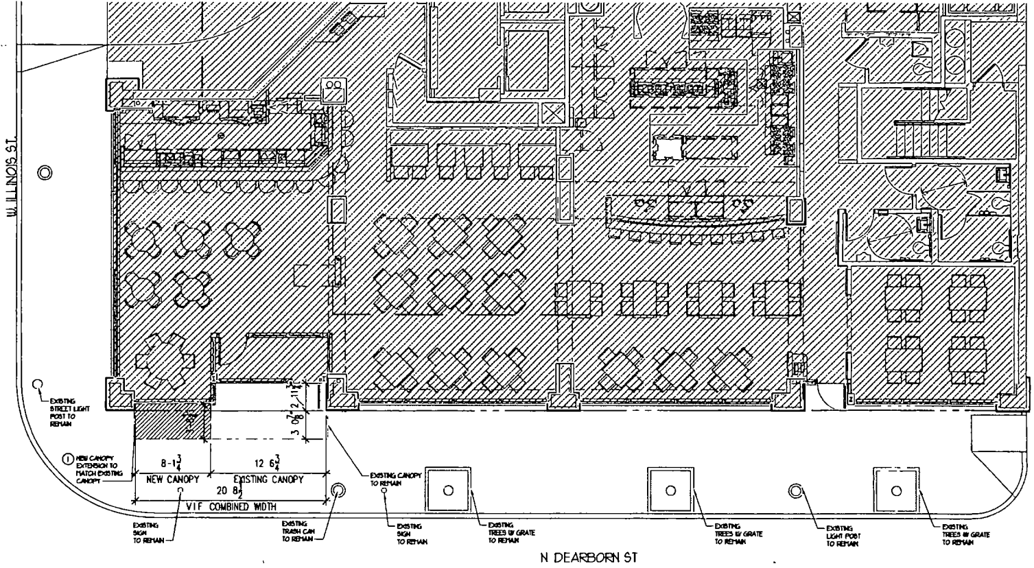
NEW CANOPY PLAN SHP - PD
