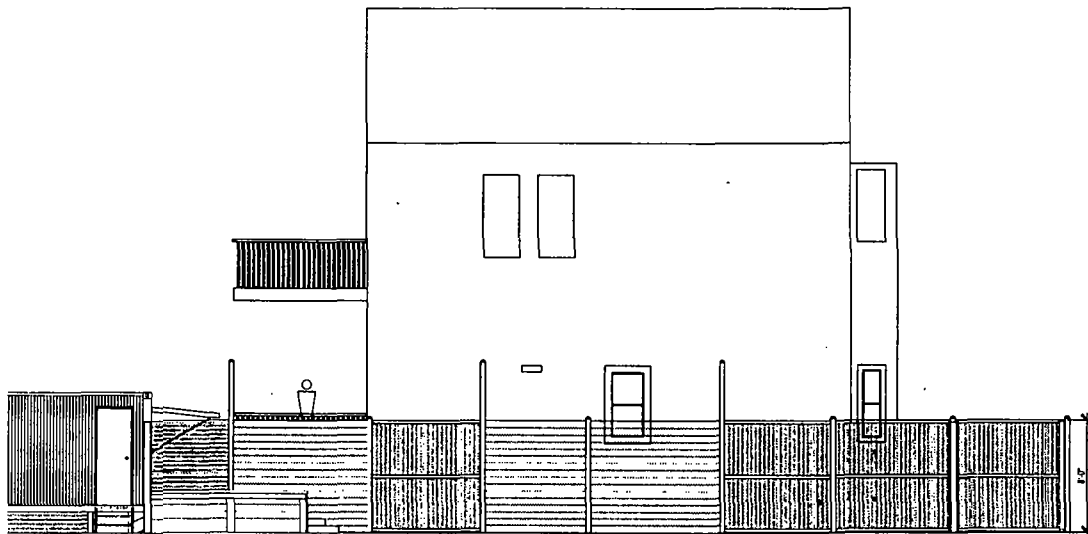
2 WEST ELEVATION @ 8 FEET SCALE: 1/4" = 1'-0"
