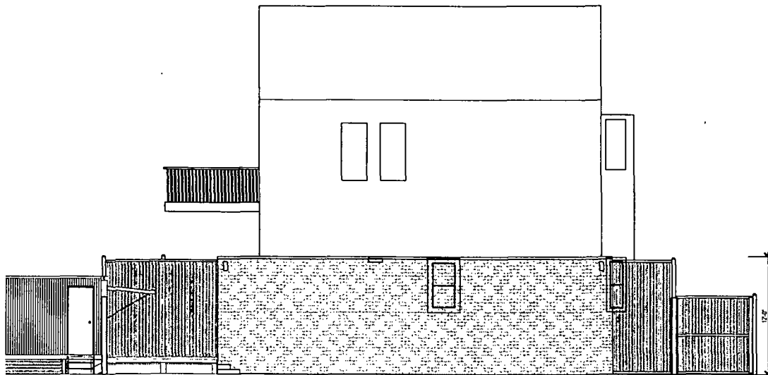
3 WEST ELEVATION @ 12 FEET SCALE: 1/4" = 1'-0"
