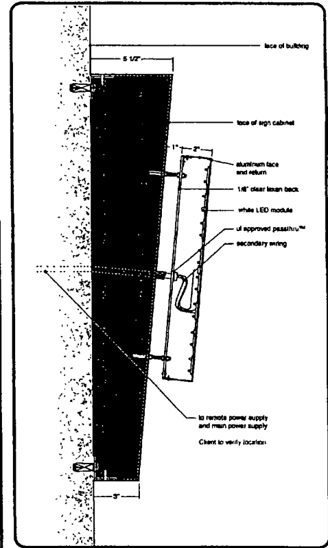
LED halo illuminated reverse panchannel letter 1 scale 1/2" = 1'-0"
