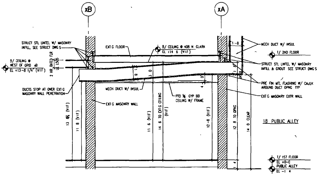
3 SECTION @ NORTH WALL DUCT PENETRATION SCALE 1/4" = 1'-0"
