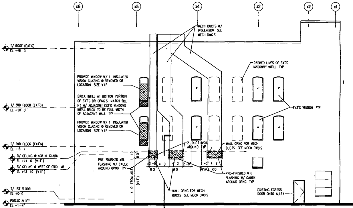
2 NORTH ELEVATION - PROPOSED SCALE 1/8" = 1'-0"
