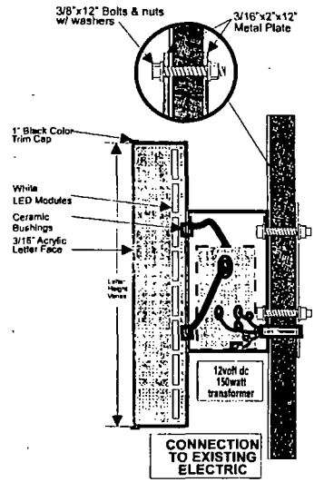
CHANNEL LETTER DETAIL NOT SCALE
