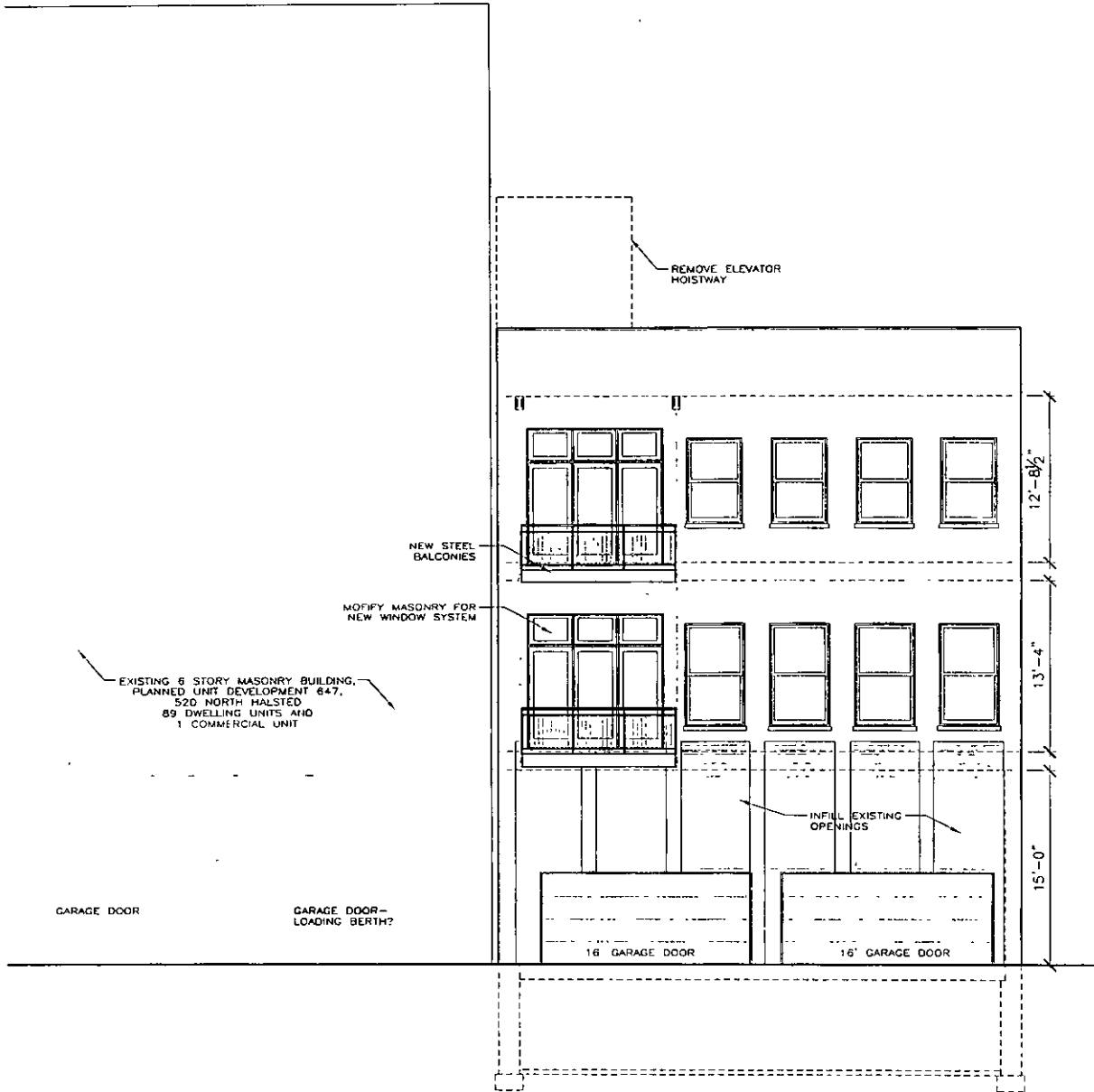
NORTH ELEVATION SCALE 1/8" = 1'-0"
