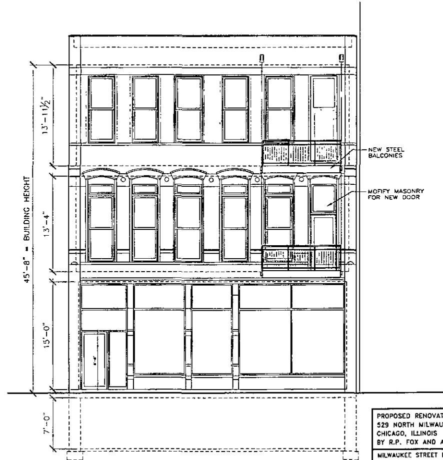
SOUTH ELEVATION SCALE 1/8" = 1'-0"
