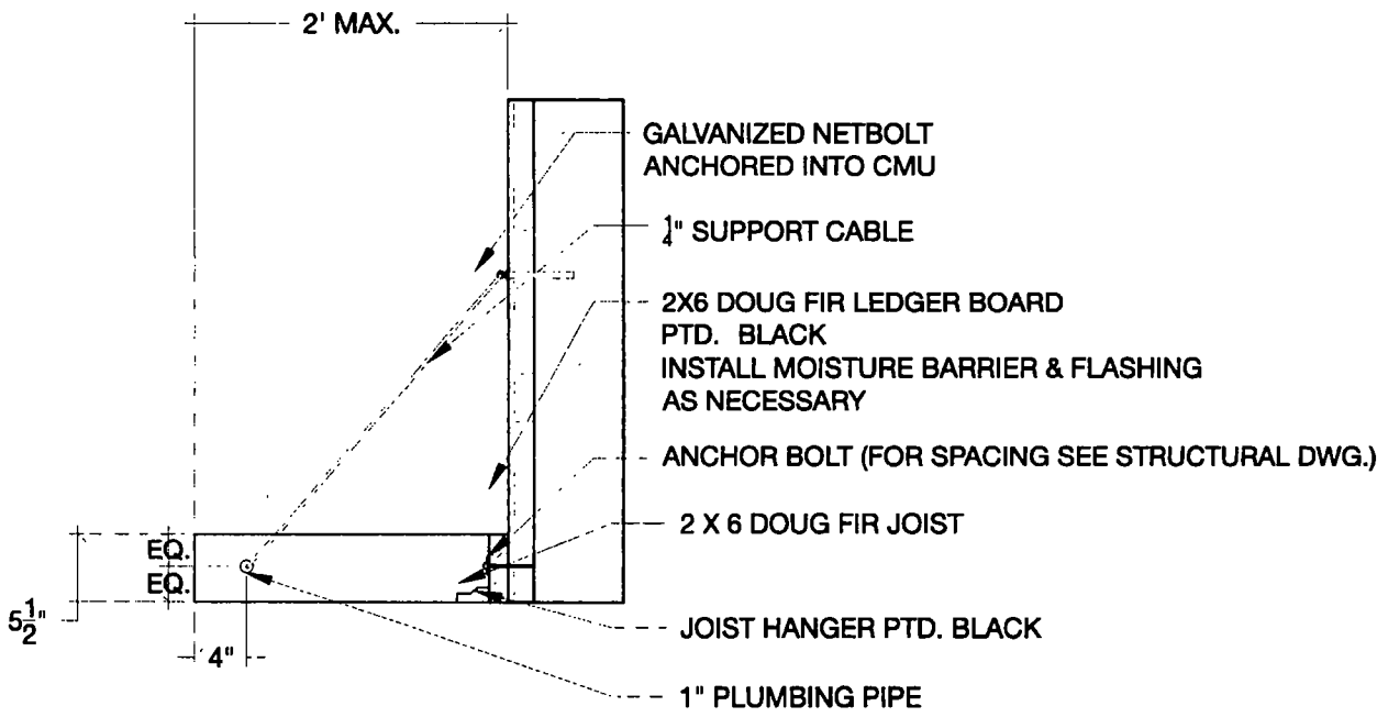
4 EXTERIOR TRELLIS DETAIL SCALE · 1" = 1'
