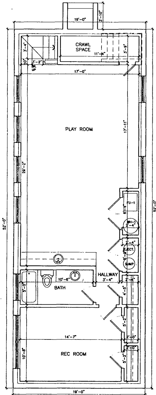
PROPOSED BASEMENT PLAN SCALE: 3/16"=1'-0" 0 2' 4' 8'
