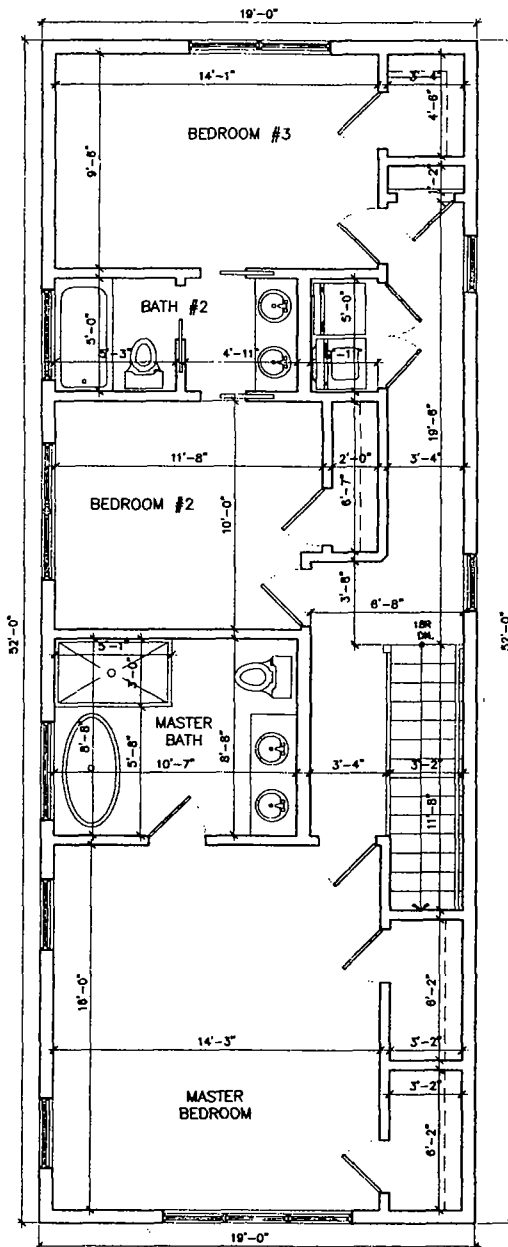
PROPOSED 2ND FLOOR PLAN SCALE: 3/16"=1'-0" 0 2' 4' 8'
