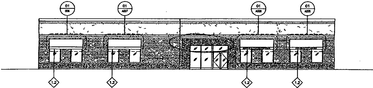
02 WEST ELEVATION - MARSHFIELD AVENUE SCALE N.T.S.
