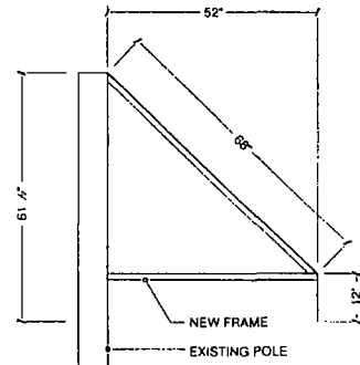
SIDE VIEW NTS
