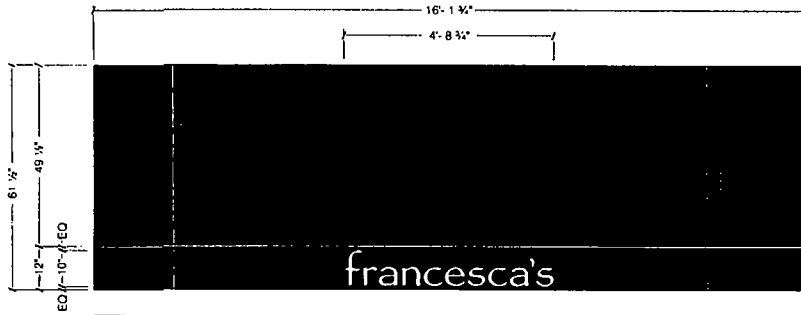
A AWNING DETAIL SCALE: 1/4" = 1'-0"
