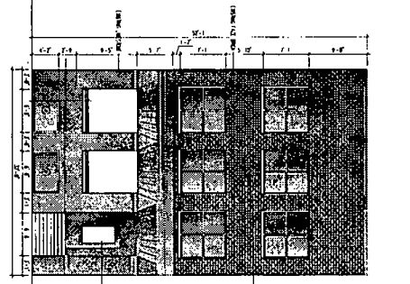
NORTH ELEVATION SCALE 1/8" = 1'-0"
