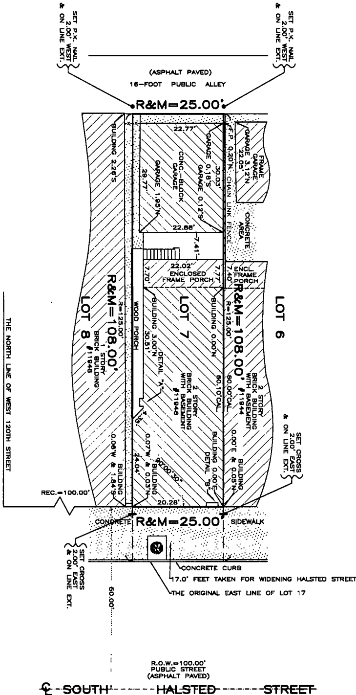
DETAIL "A" NOT TO SCALE
