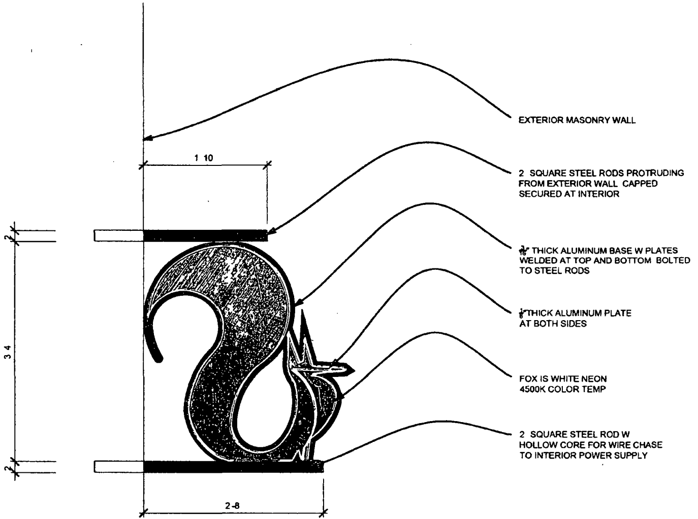
3 NEON SIGN SIDE VIEW SCALE 1 = 1'-0"
