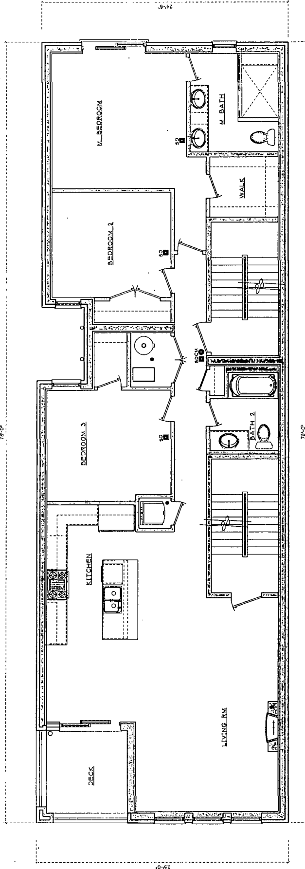
3 THIRD FLOOR PLAN SCALE 1/4" = 1'-0"
