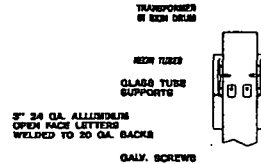
DOUBLE-FACE SIGN CROSS SECTION
