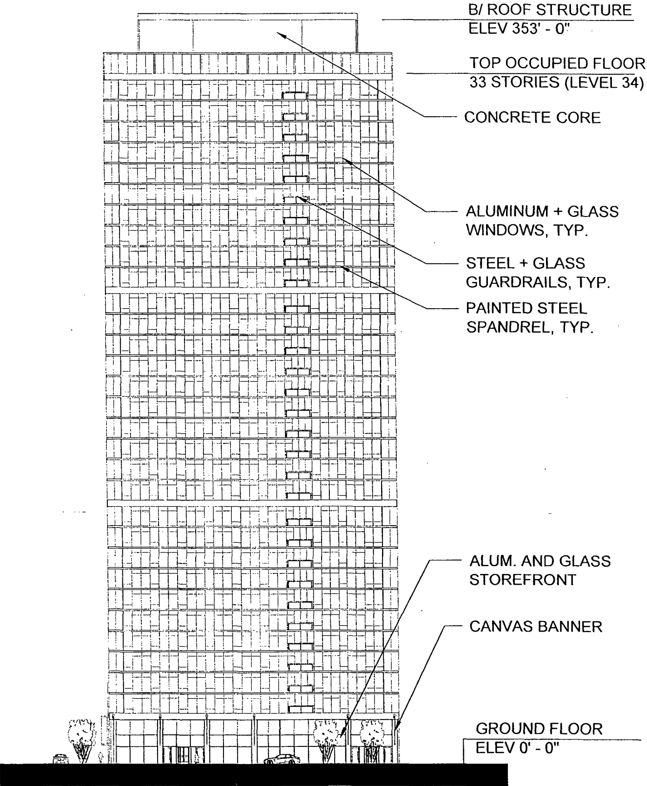
H1. SOUTH ELEVATION ALONG CHICAGO AVENUE
