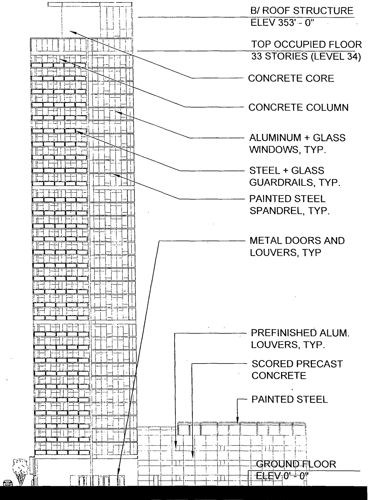
H3. EAST ELEVATION ALONG ALLEY
