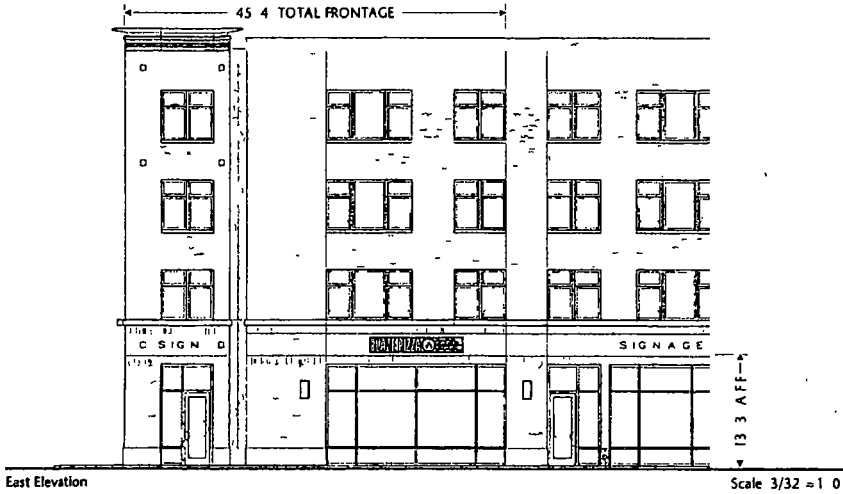
East Elevation
