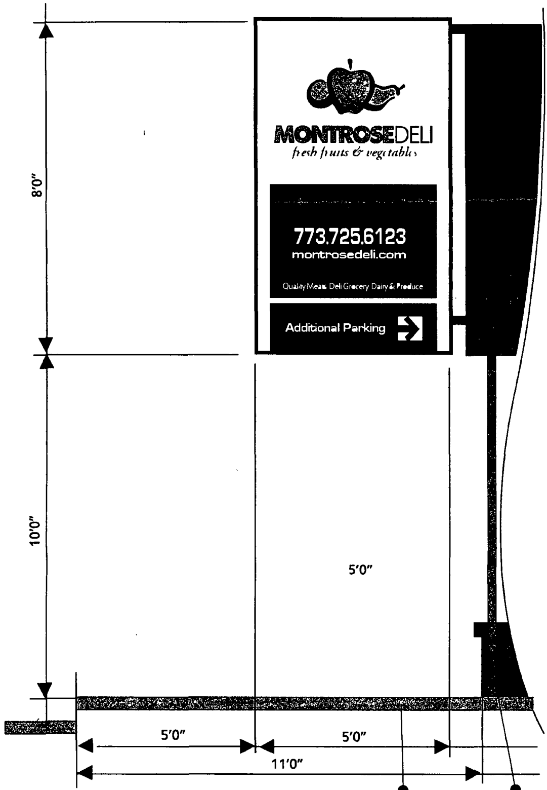
DOUBLE SIDED 5'0"X8'0" ELECTRIC SIGN
