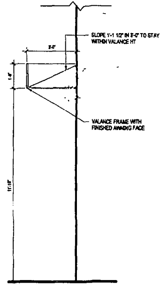
SECTION
