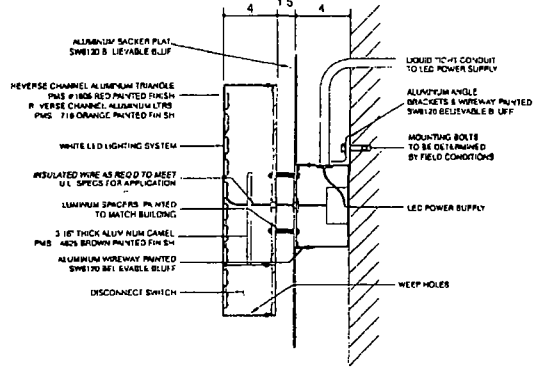
SECTION DETAILS 1/4\"/>
