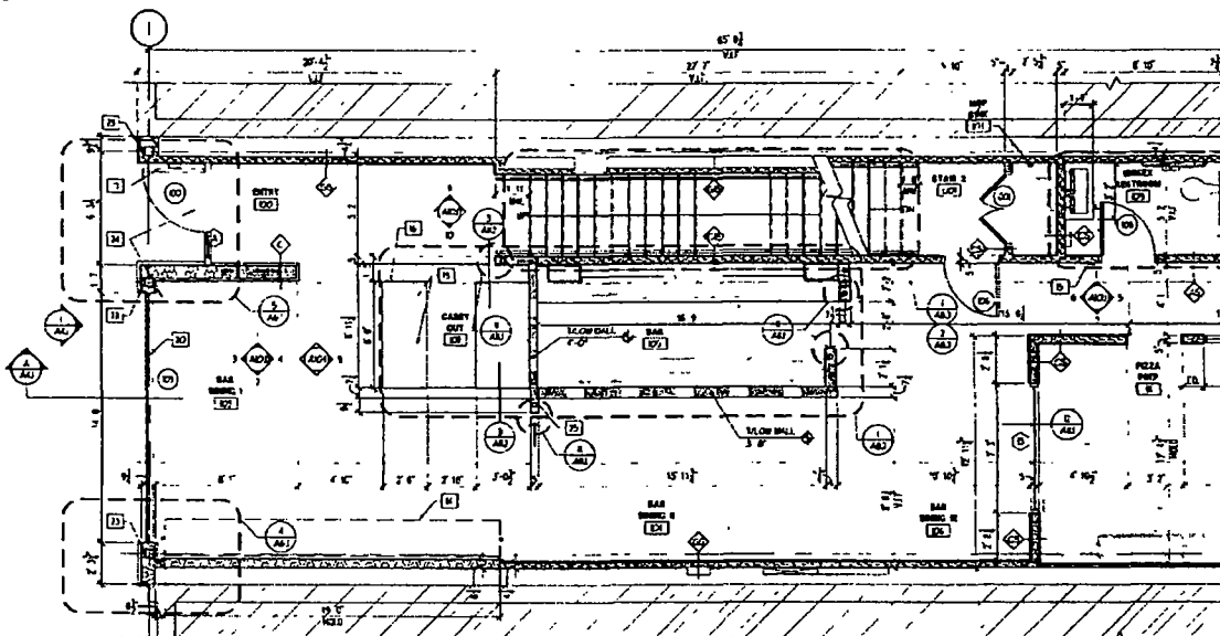
2 GROUND LEVEL FLOOR PLAN 4" = 1'-0"
