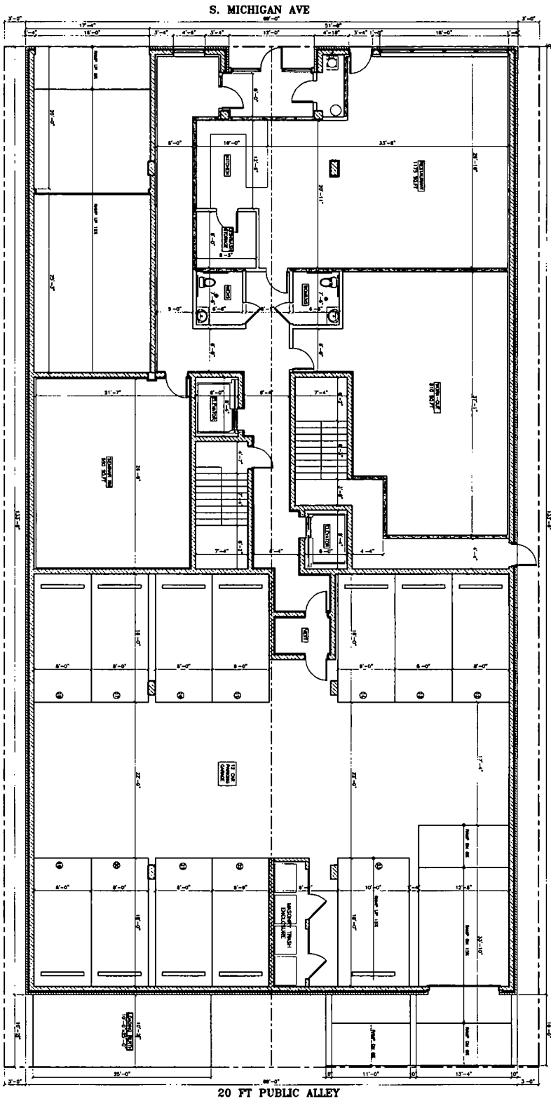
⊕ FIRST FLOOR PLAN SCALE: 1/8" = 1'-0"
